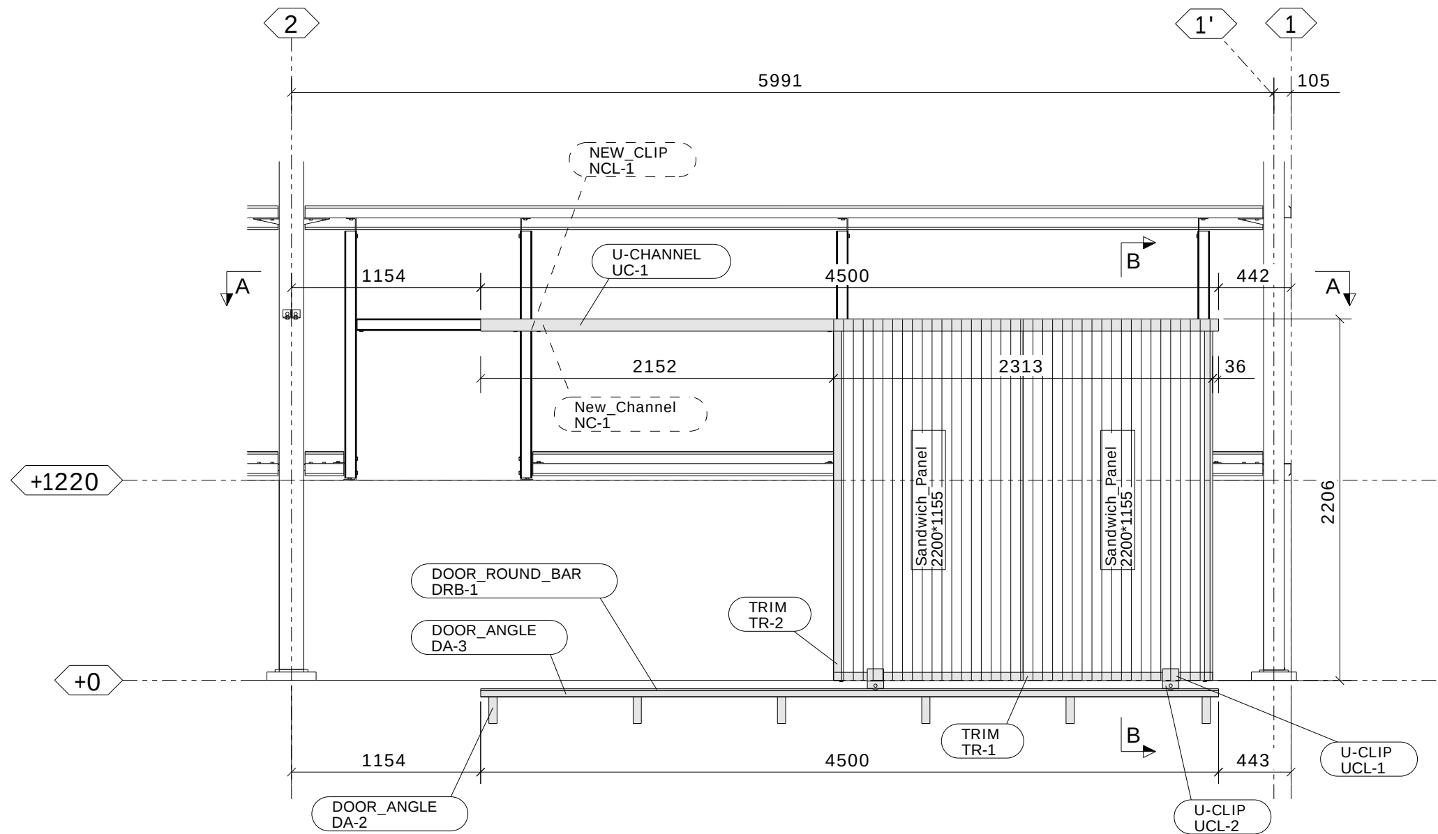
SINGLE SLIDING DOOR ELEVATION
